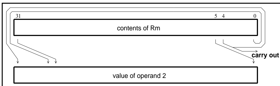
Figure 5-9: Rotate right
