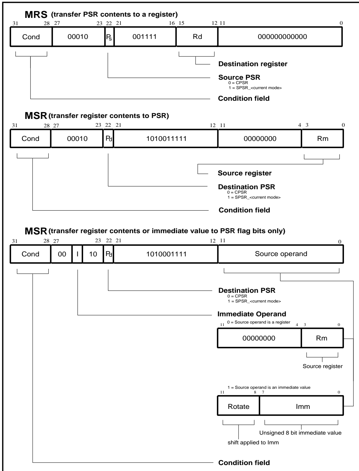
Figure 5-12: PSR transfer
