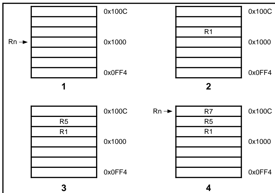
Figure 5-18: Pre-increment addressing
