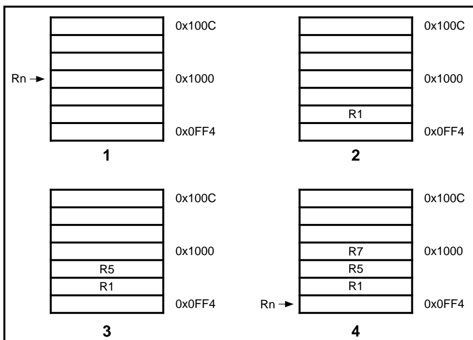
Figure 5-19: Post-decrement addressing
