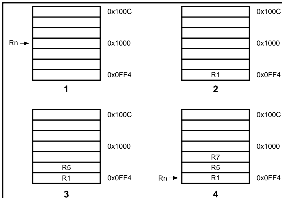
Figure 5-20: Pre-decrement addressing
