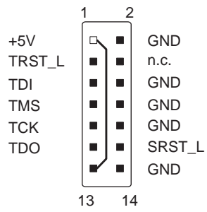
Figure A-10 JTAG Connector J1 Pinout
