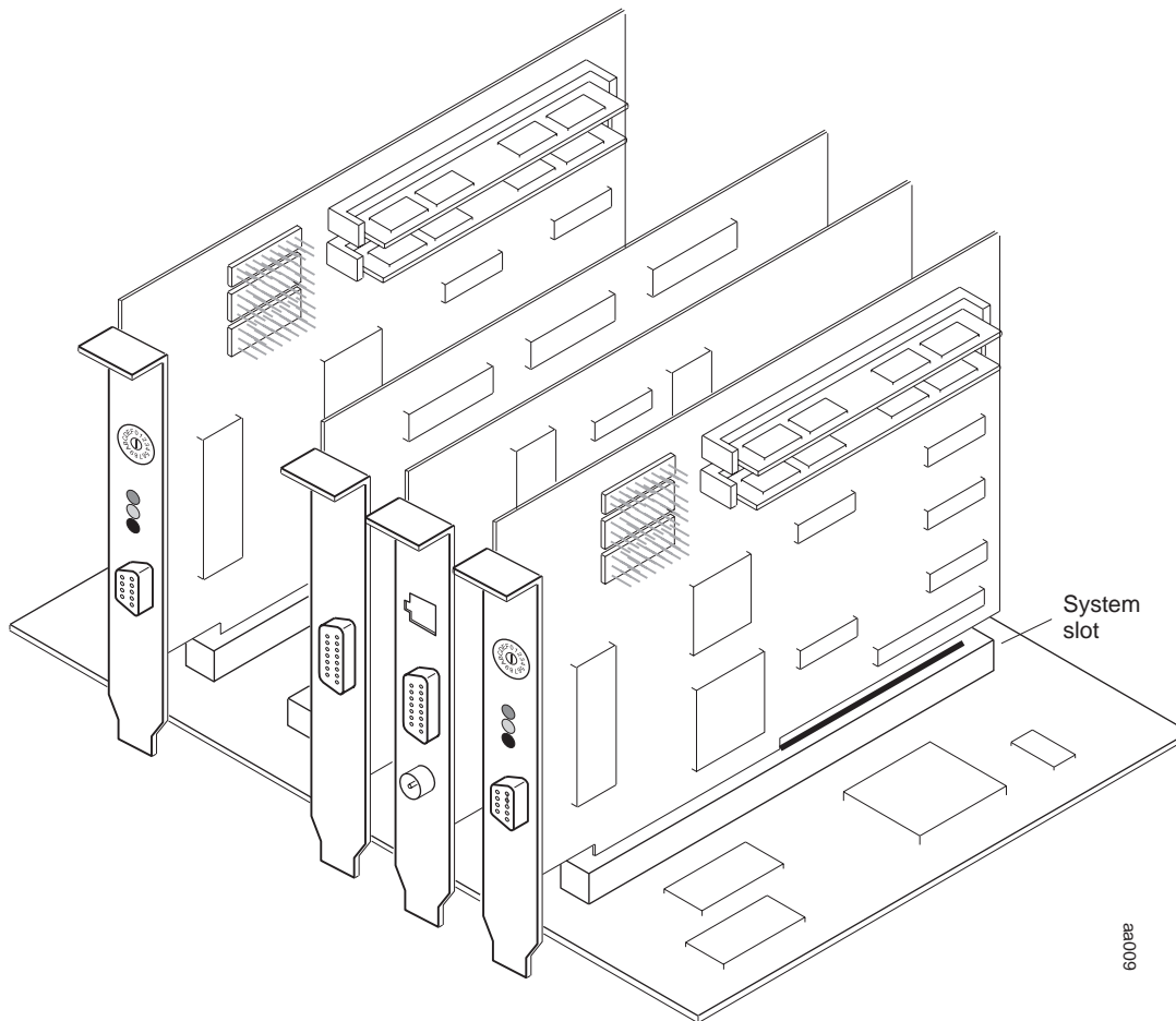
Figure 1–2 Example Configuration in an EBSA-BPL-5V or EBSA-BPL-3V3 Backplane
