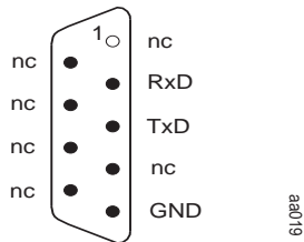
Figure A–9 Serial Port Connector Detail
