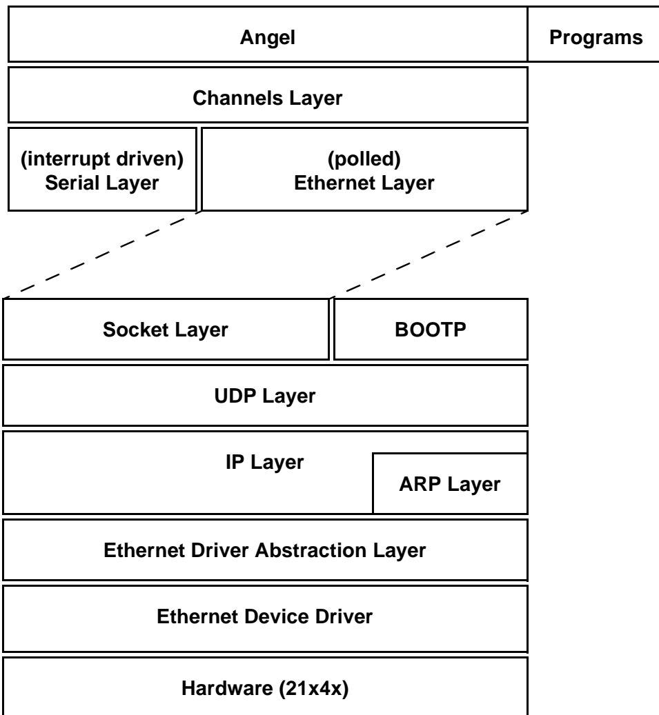
Figure 1–3 Angel Communication Overview
