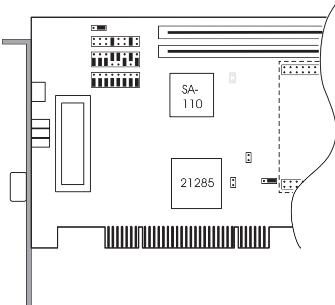
Figure A-4 EBSA-285 Configured as a Host Bridge
