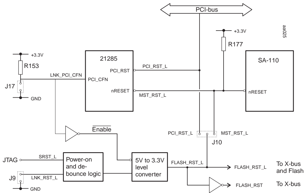
Figure 8–1 Reset Circuits
