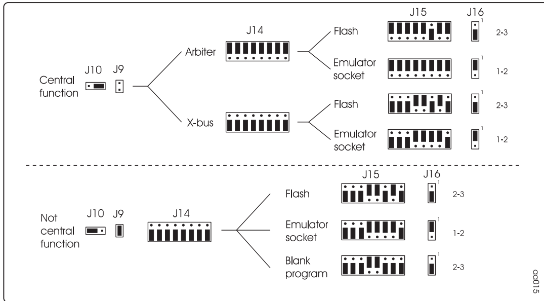
Figure A-2 Primary Jumper Settings
