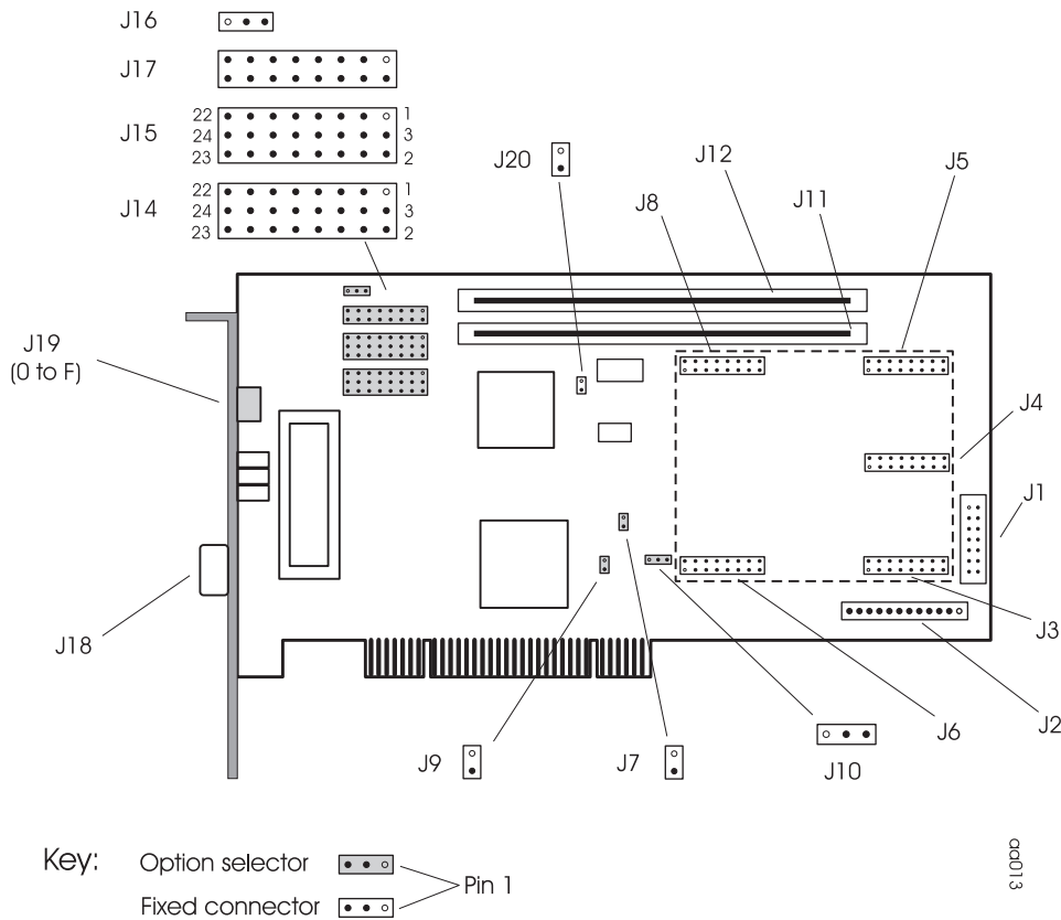
Figure A-1 Jumper and Connector Locations
