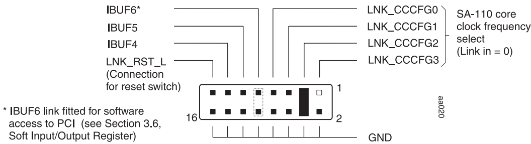
Figure A-6 J17 Pinout Showing Default Jumper Configuration
