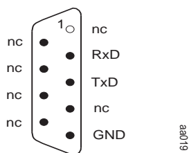
Figure A–9 Serial Port Connector Detail
