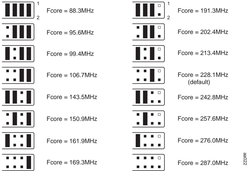
Figure A-7 J17 Core Clock Selection Jumpers
