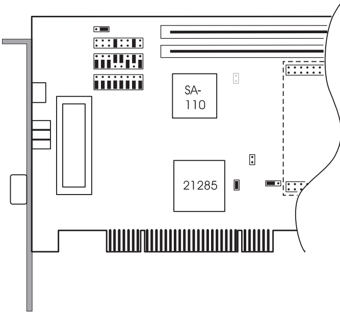
Figure A-3 EBSA-285 Configured as an Add-in Card
