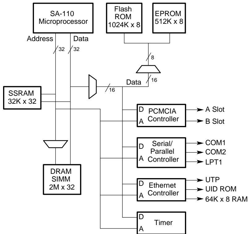
Figure 1 EBSA-110 Evaluation Board Block Diagram
