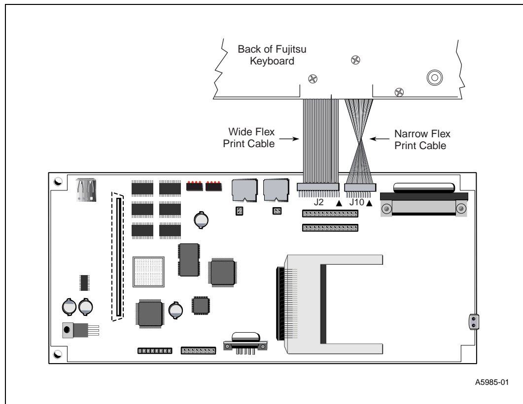
Figure 3-5. Keyboard Connectors
