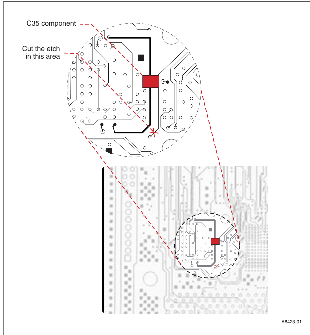
Figure 1. Etch Cut under C35
