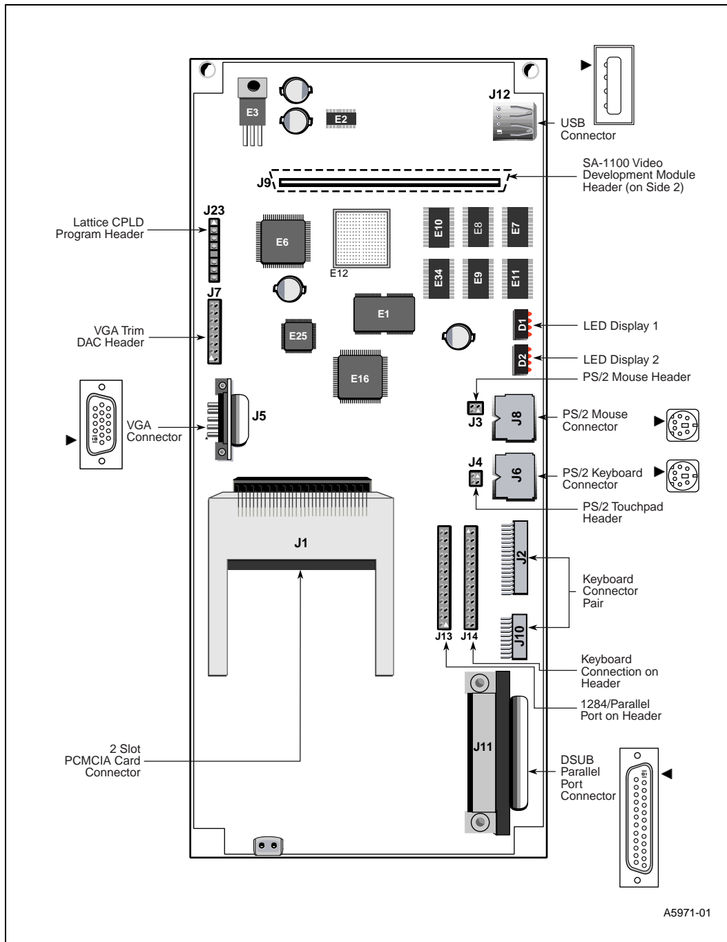
Figure 3-2. SA-1101 Development Board
