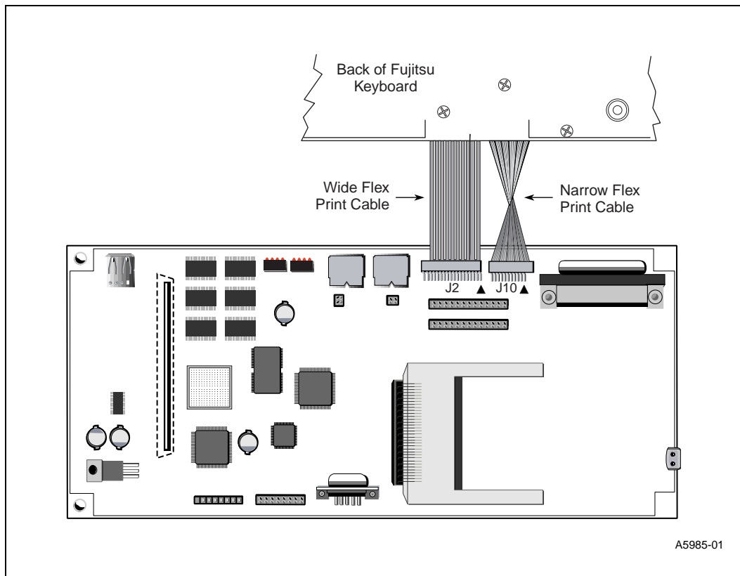
Figure 2. Keyboard Connectors
