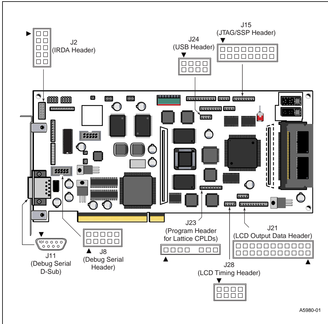
Figure A-6. IrDA, JTAG, LCD, and Debug Ports and Headers
