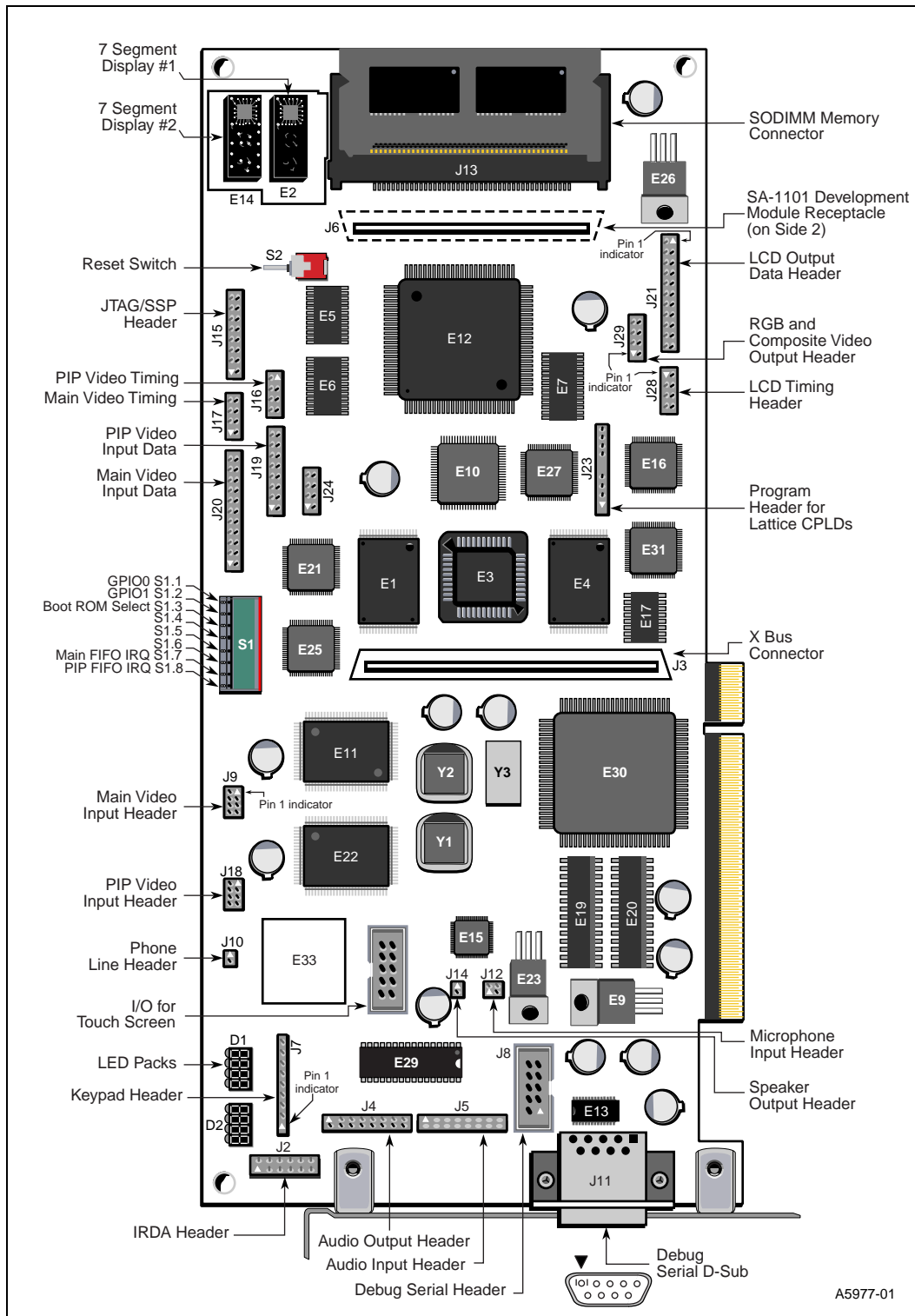
Figure 3-1. SA-1100 Multimedia Development Board
