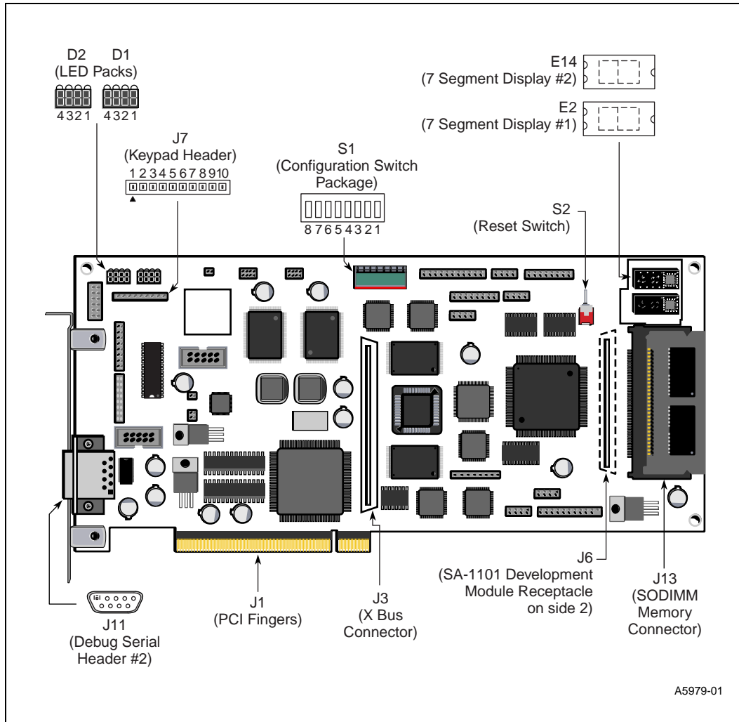
Figure A-2. S1, S2, LEDs, Keypad, Debug, X Bus, Daughter Card and SODIMM Connector
