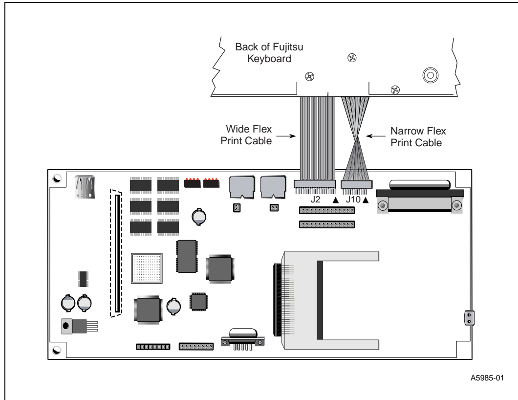
Figure B-3. Keyboard Connectors
